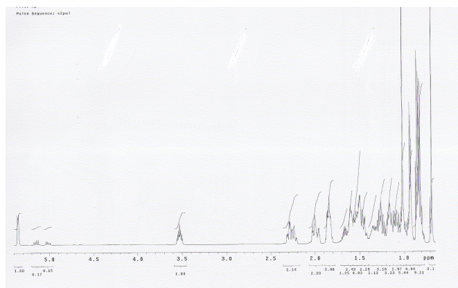
Fig. 1 1 H NMR spectrum of \beta -Sitosterol (1) with proton integration
