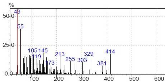
Fig. 3a Mass spectrum of \beta -sitosterol (1)
