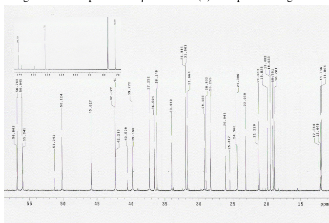
Fig. 2 13 C NMR spectrum of \beta -Sitosterol (1)
