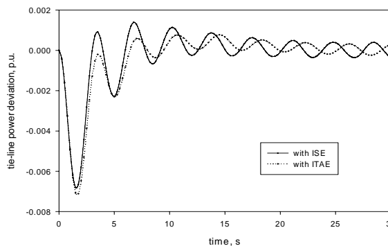
Fig. 7 (c) Tie-line power deviation in area-1
