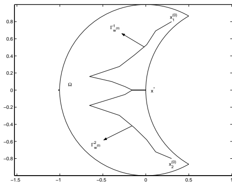
Fig. 1. The homotopy pathways of Example 1
