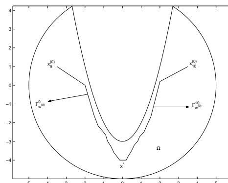
Fig. 5. The homotopy pathways of Example 5
