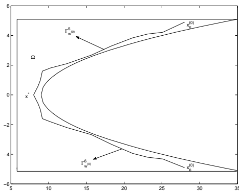
Fig. 3. The homotopy pathways of Example 3
