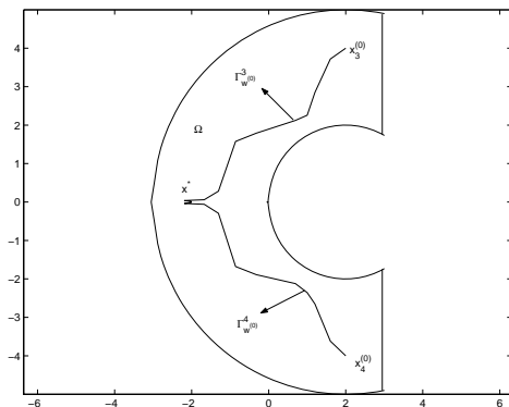
Fig. 2. The homotopy pathways of Example 2
