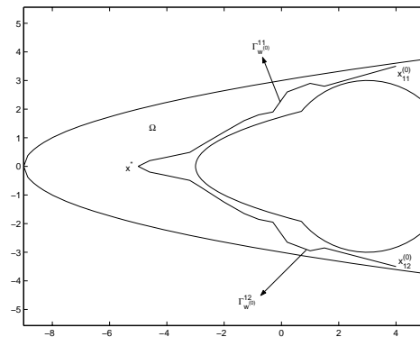
Fig. 6. The homotopy pathways of Example 6
