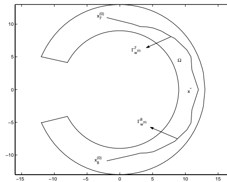
Fig. 4. The homotopy pathways of Example 4
