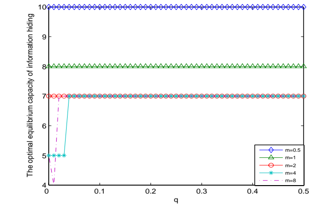
Fig. 3. The optimal equilibrium capacity of information hiding for r=8 , R=2 , F=6 , g=2 , \lambda=1 , x=0.6 .
