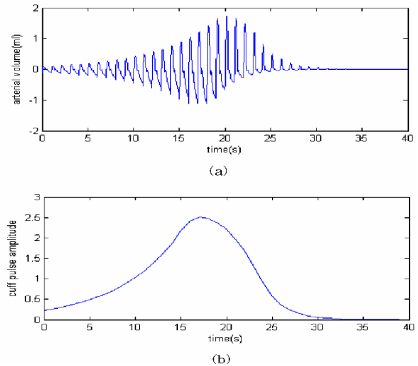
Fig. 5 The procedure acquisitioning of the oscillometric waveform: (a) oscillation waveform removed DC component in Fig. 4 and (b) oscillometric waveform
