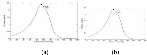
Fig. 6 Output oscillometric waveform of the arterial pressure-volume model: (a) model input signal is Fig. 3 (a) and (b) model input signal is Fig. 3 (b)
