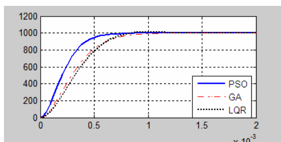
Fig. 7 Comparison between GA, LQR and PSO based PID control in speed control of LBDC motor
