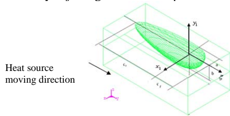
Fig. 5 Double elliptic function model
