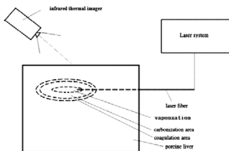
Fig. 1 Schematic diagram of conducting the experiment
