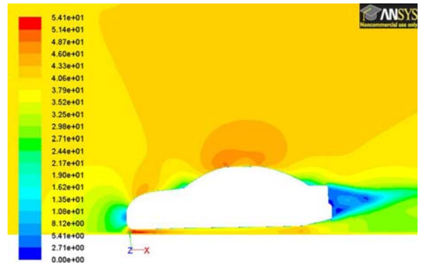
Fig. 4 Distribution of Velocity on the symmetry plane
