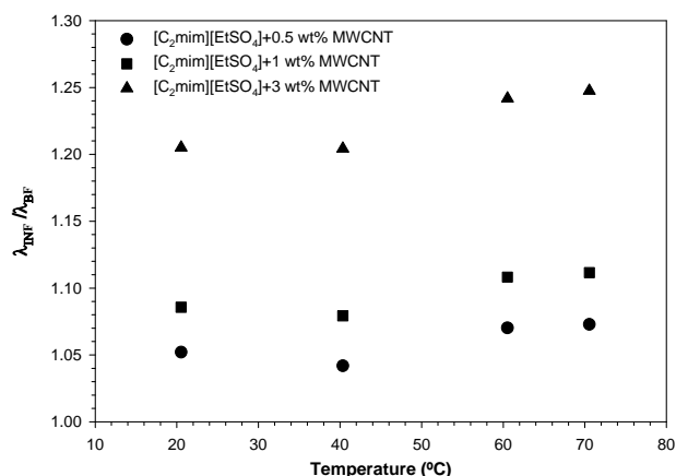
Fig. 3 Temperature-dependent thermal conductivity of ionanofluids [20]
