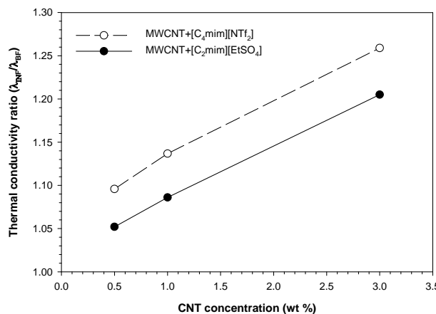
Fig. 2 Enhancement of thermal conductivity of ionanofluids as a function of CNT concentration at room temperature [18]
