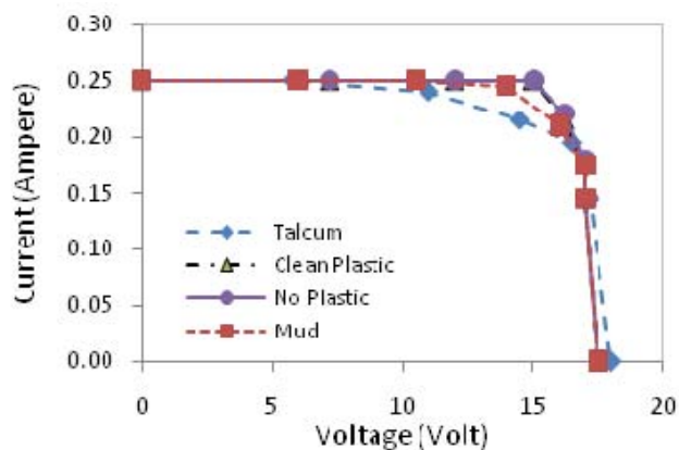
Fig. 8 I-V characteristics for irradiation of 301 W/m 2
