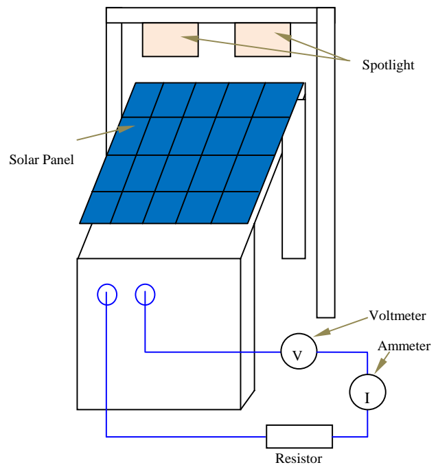
Fig. 1 Schematic of the system
