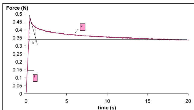
Fig. 4 Hair relaxation curve.
