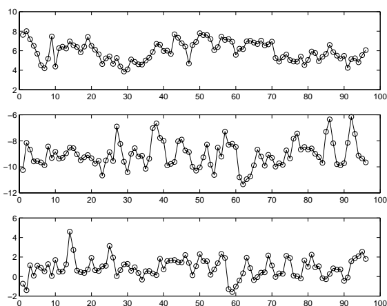
Fig. 4. Estimated sources
