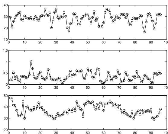
Fig. 2. Original sources
