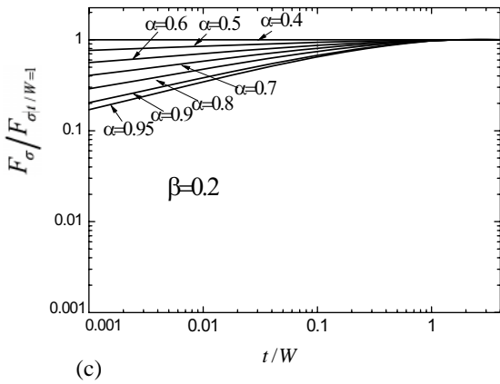
Fig.8 F_{\sigma}/F_{\sigma t/W=1} with varying adhesive thickness t/W in Fig.1 (a) for (a) \beta=-0.1 (b) \beta=0 , (c) \beta=0.2
