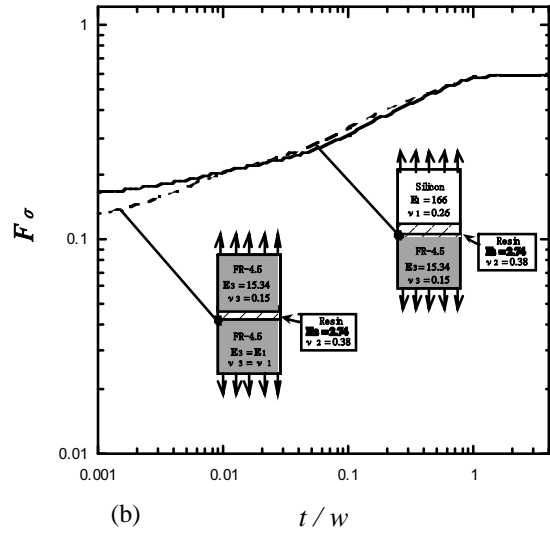
Fig.10 Comparison between the effects of adhesive thickness on the results for different adherents and the same adherents for example 2 material combination (a) the upper corner (b) the lower corner
