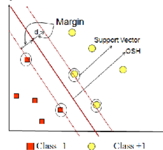
Fig. 2 Support vector and optimum separating hyperplane
