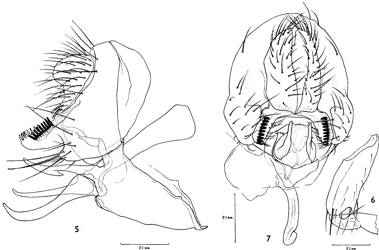
FIG. 5.— D. silvestris Basden. Male genitalia, side view. From paratype specimen. (Liberton, Edinburgh, Scotland.) Note "barbed" pincer.
