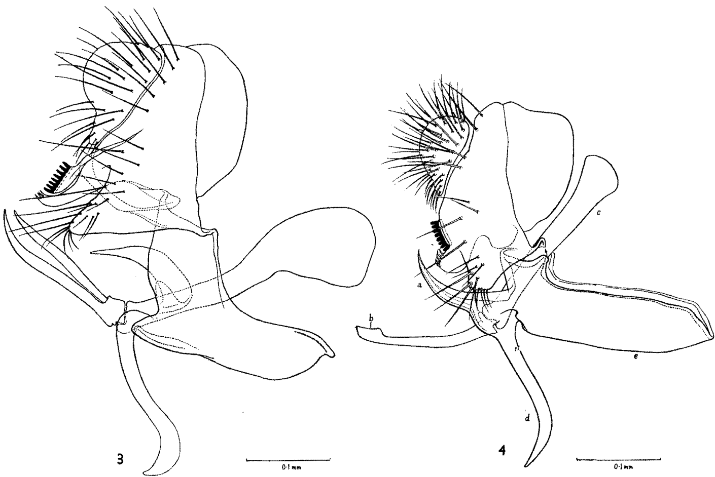
FIG. 3.— Drosophila obscura Fallén. Male genitalia, side view. (Furuffaten.) Note the bifid penis, the broad-ended lancet process, and the short hypandrium.
