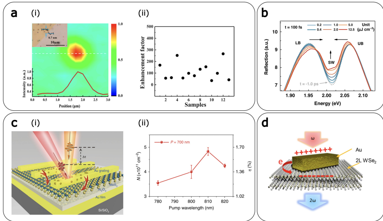
FIG. 12. Application of ultrafast plasmonics in low-dimensional semiconductors. (a-i) Normalized SHG intensity map of a monolayer \text{WS}_2 integrated in a plasmonic nanocavity with a scanning step of 200 nm. The curve is the SHG intensity line profile along the white dashed line. Inset shows an optical micrograph of the hybrid system where the black dots are the Ag nanocubes. (ii) SHG enhancement factor with different Ag nanocubes under fixed excitation laser with wavelength of 820 nm. 403 Reproduced with permission from Han et al. , ACS Photonics 7, 562 (2020). Copyright 2020 American Chemical Society. (b) Transient reflection spectra of the \text{WS}_2/\text{Au} -nanodiscs plexciton system measured at 100 fs at different fluence rate. The gray dashed line is the unaffected probe spectrum by probe pulse at -1 ps. 417 Reproduced with permission from Tang et al. , Light: Sci. Appl. 11, 94 (2022). Copyright 2022 Author(s), licensed under a Creative Commons Attribution (CC BY) license. (c-i) Schematic of pump-probe measurements on Au grating/ \text{MoS}_2/\text{Al}_2\text{O}_3/\text{Au} sandwiched heterostructure to demonstrate plasmonic hot electron transfer from a gold grating to the \text{MoS}_2 monolayer. (ii) Pump wavelength dependent injected hot electron densities using the previous setup from (d) and corresponding efficiency for the heterostructure with 700 nm grating period. 421 Reproduced with permission from Shan et al. , Light: Sci. Appl. 8, 9 (2019). Copyright 2016 Author(s), licensed under a Creative Commons Attribution (CC BY) license. (d) A diagrammatic model to describe the hot electron induced symmetry breaking and probing SHG in a Au/2L \text{WSe}_2 hybrid system. 422 Reproduced with permission from Wen et al. , Nano Lett. 18, 1686 (2018). Copyright 2018 American Chemical Society.
