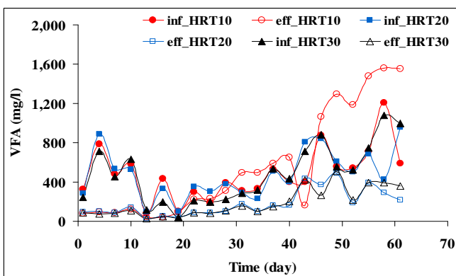
Fig. 6 Volatile fatty acid during the CSTR operation
