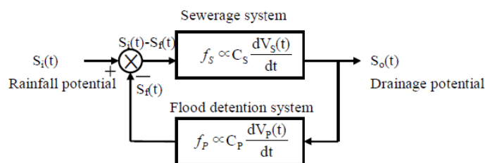
Fig.4 The stable flood detention model (SFD model)
