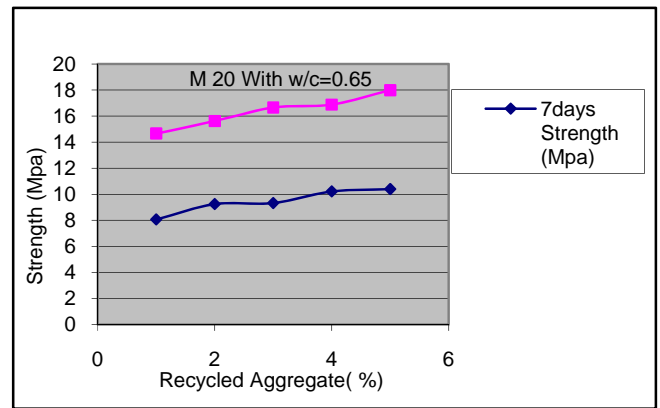
Fig. 9 Compressive strength at 7days & 28 days of M20 concrete with w/c=0.65
