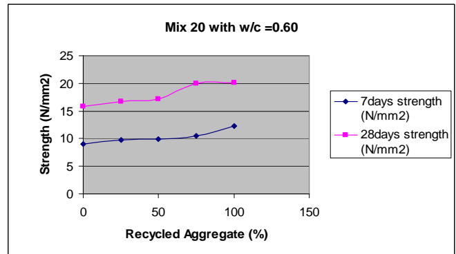
Fig. 8 Compressive strength at 7days & 28 days of M20 concrete with w/c=0.60
