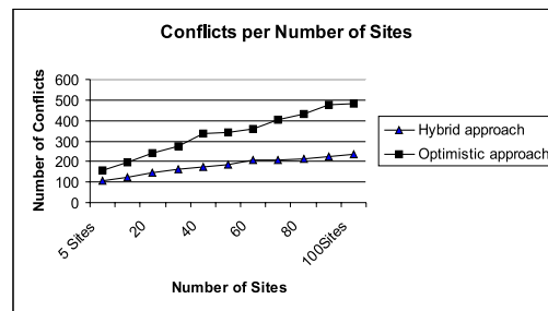
Fig. 5. Conflicts count by sites number
