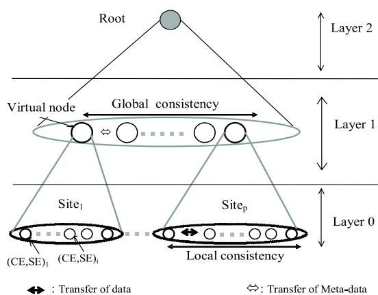
Fig. 2. Multi Layer Model Architecture
