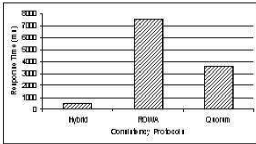
Fig. 7. Average response time of 20 Sites
