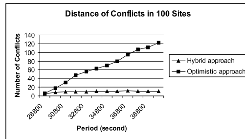
Fig. 6. Distance by Period
