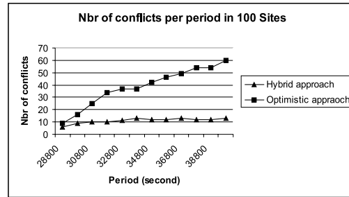
Fig. 4. Count conflicts by period
