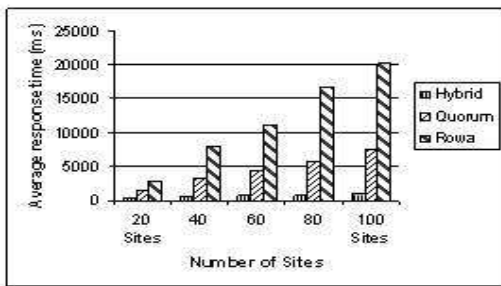
Fig. 8. Average response time per number of sites
