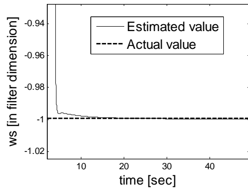
Fig. 6 Estimation of frequency of sloshing in flight time
