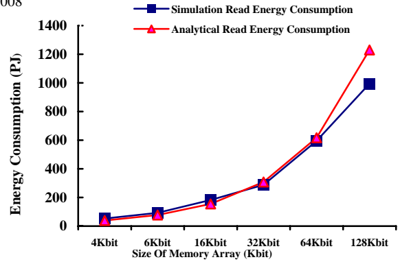
Fig. 4 Simulation and analytical read energy consumption
