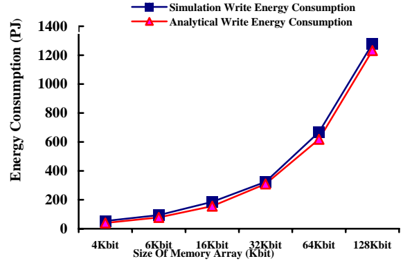
Fig. 5 Simulation and analytical write energy consumption
