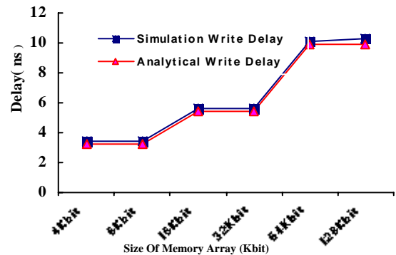
Fig. 7 Simulation and analytical write delay
