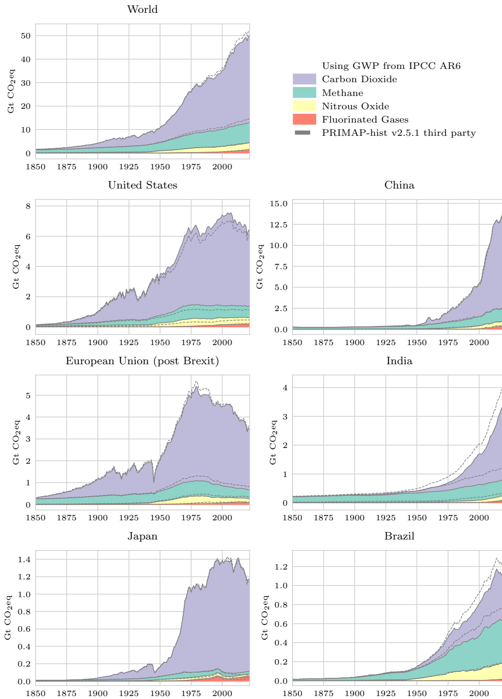
PRIMAP-hist v2.5.1 country reported priority data by gas for major emitters.
