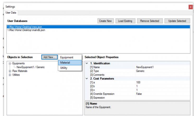
Fig. 5: Method tab
