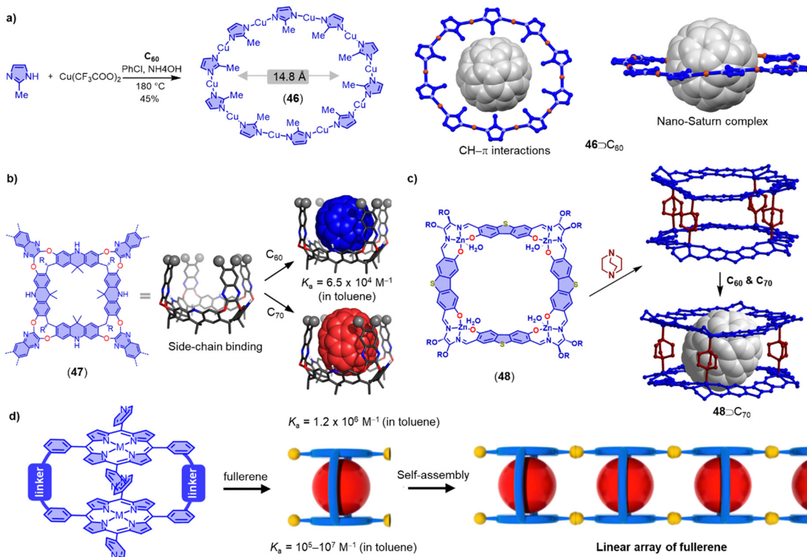
Fig. 14 (a) Selective synthesis of [Cu_{10}(2\text{-methylimidazole})_{10}] 46 utilizing C_{60} as the template, and the solid-state structure of nano-Saturn complex 46 \rightarrow C_{60} . (b) Molecular models of megalo-cavitands 47 and corresponding C_{60} and C_{70} complexes. Adapted from ref. 271 with permission from Wiley-VCH, copyright 2022. (c) Synthesis of a supramolecular double-decker cage 48 and its selective recognition with C_{70} . (d) Formation of linear array of fullerenes in self-assembled porphyrin nanotube. Adapted from ref. 272 with permission from American Chemical Society, copyright 2014.
