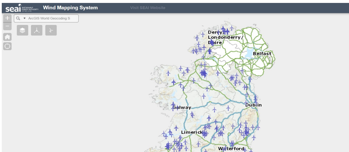
Figure 7 SEAI's Wind Atlas of Irish's windfarms
