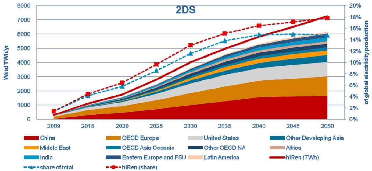
Figure 2 Wind power deployment to 2050 in the Roadmap vision (Darwish & Al-Dabbagh, 2020)
