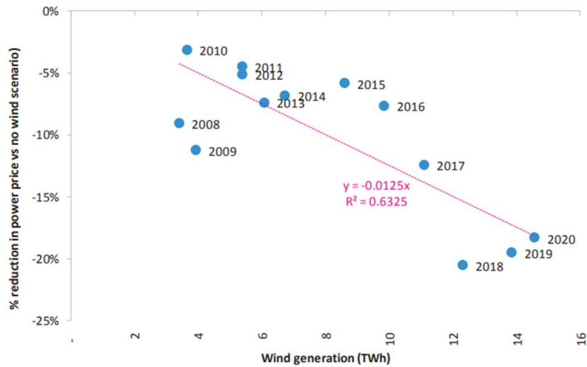
Figure 32 Wind generation and wholesale price reduction vs ‘no wind’ scenario (Baringa, 2020)
