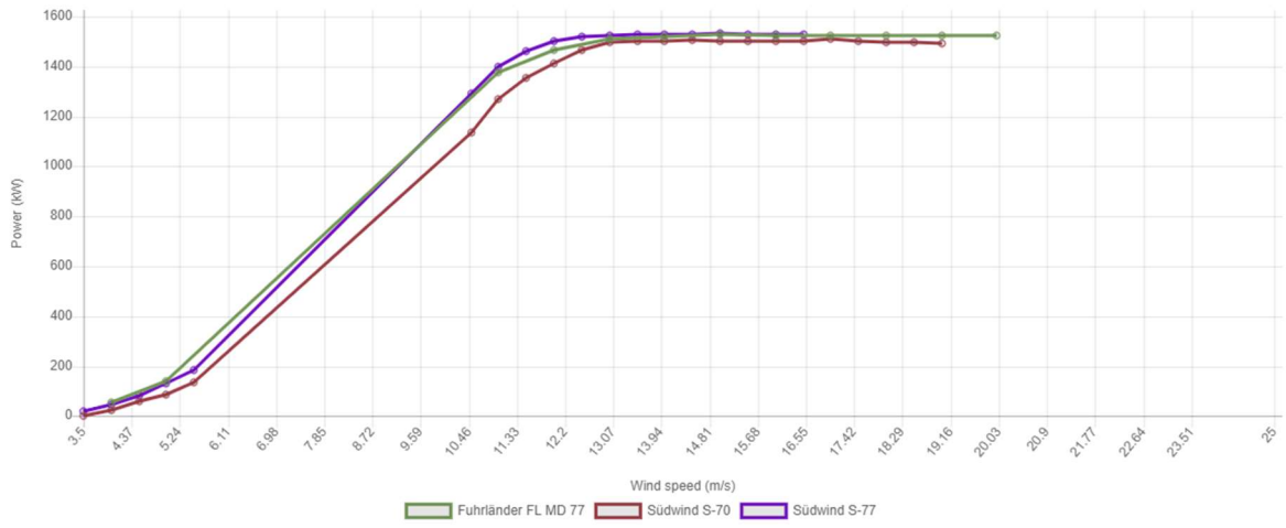
Figure 14 Power curve of the three wind turbine models
