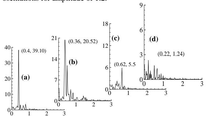
Fig. 11 Vertical velocity spectra at X/D = 2.5 for different amplitude: (a) 0.15, (b) 0.6, (c) 0.9 and (d) 1.2
