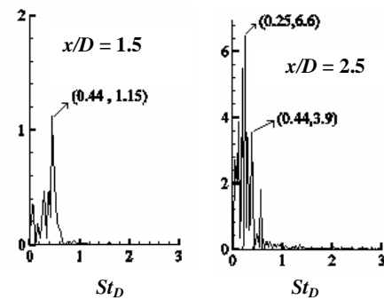
Fig. 10 Velocity spectra at two locations without control
