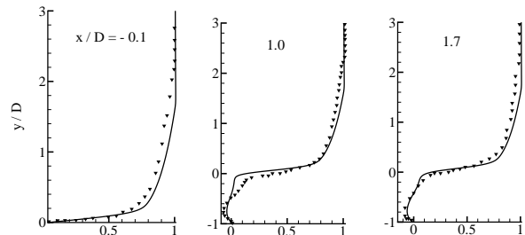
Fig. 5 Comparison of mean velocity profiles with experiment of Pereira And Sousa [6] Present LES ——— and experiment ▼▼▼
