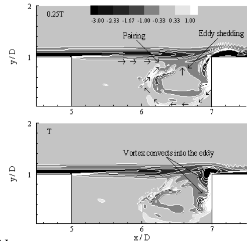
Fig. 3 Instantaneous vorticity contours illustrating pairing and eddy shedding
