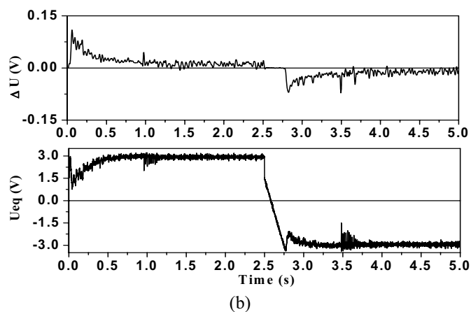
Fig. 10 Experimental results of position control (a) displacement and voltage commands of the piezo-VCM actuators, (b) \Delta U , and equivalent control U_{eq} .
