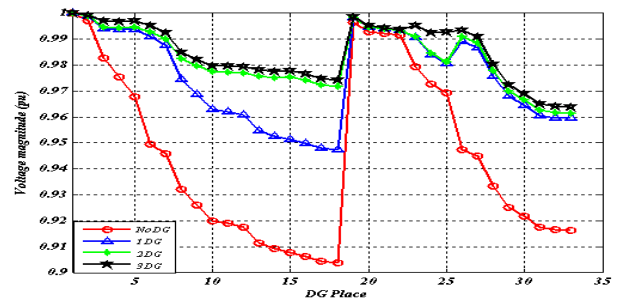
Fig. 5. Voltage profile of 33-bus test system in presence of type 1 DG unit(s)
