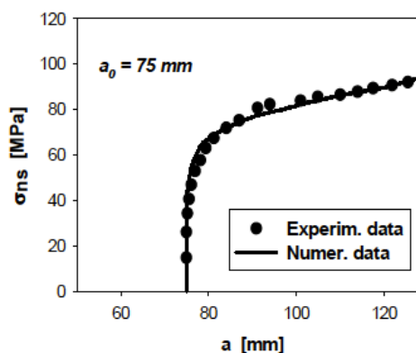
Fig. 5 Stress vs. Half crack length
