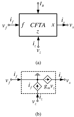
Fig. 1 CFTA (a) Symbol (b) Equivalent circuit
