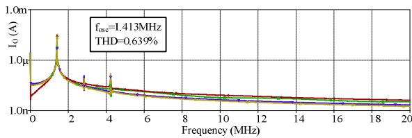
Fig. 9 Spectrum of signal in Fig. 8
