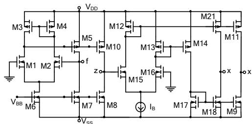
Fig. 2 Schematic of the CMOS CFTA
