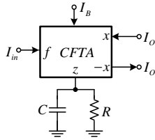
Fig. 4 CFTA-based current-mode lossy integrator
