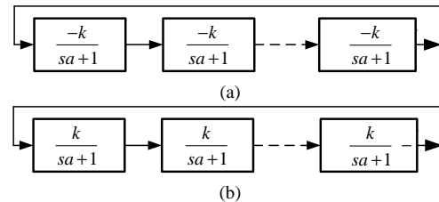
Fig. 3 MSO block diagram for (a) odd phase (b) odd/even phase
