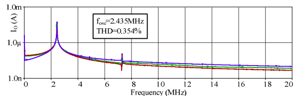
Fig. 7 Spectrum of signal in Fig. 6
