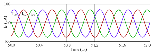
Fig. 6 Current outputs of the proposed MSO ( n=3 )
