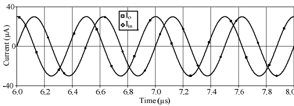
Fig. 6 Filter response to a 2MHz sinusoidal input signal
