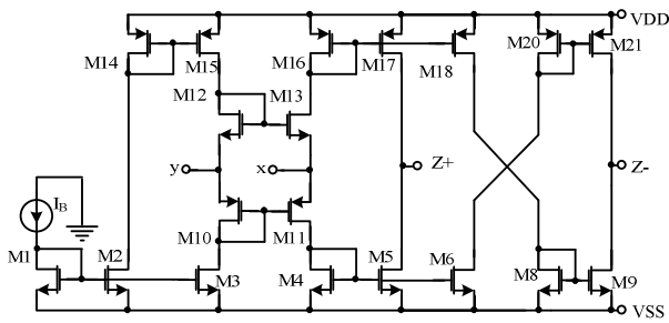
Fig. 2 Schematic of the CMOS CCCII
