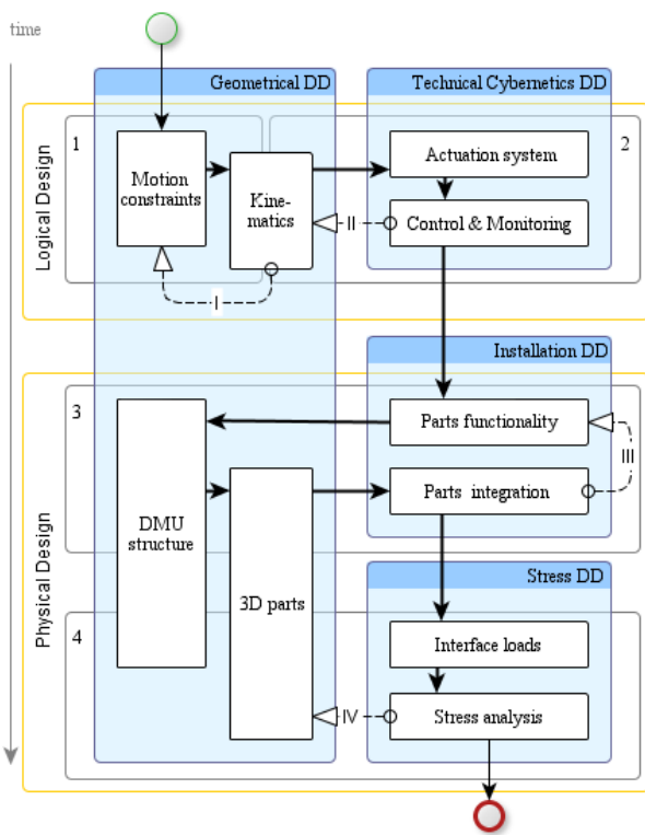
Fig. 6 Concept for a multidisciplinary design process
