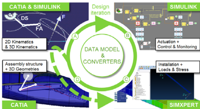
Fig. 7 Example for a multidisciplinary model-based tool chain
