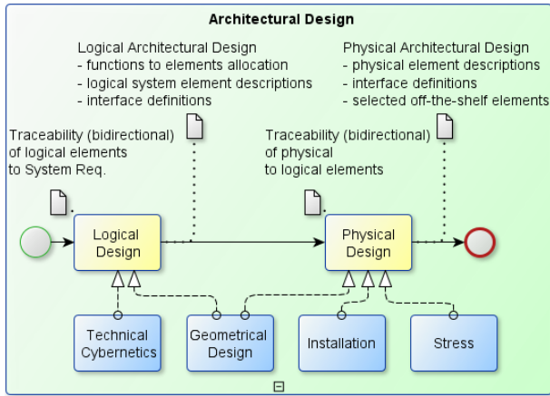
Fig. 4 Stage decomposition and split of engineering domains
