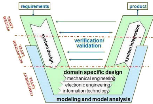
Fig. 2 Design methodology for mechatronics systems as Vee diagram as proposed by VDI 2206 [11]
