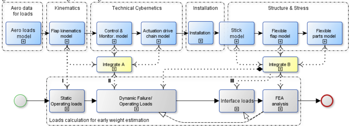
Fig. 8 Example for multidisciplinary loads calculation sequence
