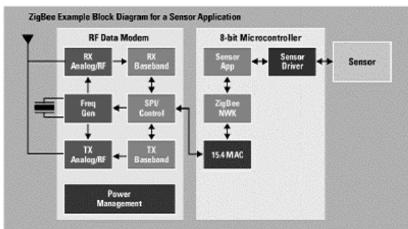
Fig. 7. ZigBee system.
