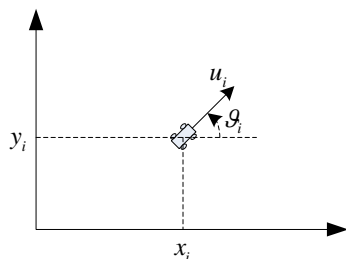
Fig. 2. Nonholonomic robot.
