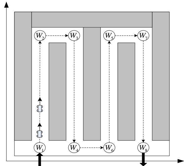
Fig. 3. Greenhouse ground plan.
