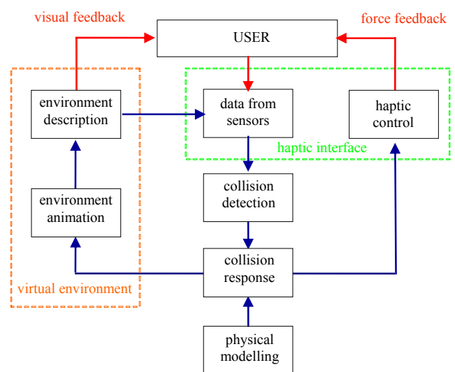
Fig. 1 Scheme of the simulator
