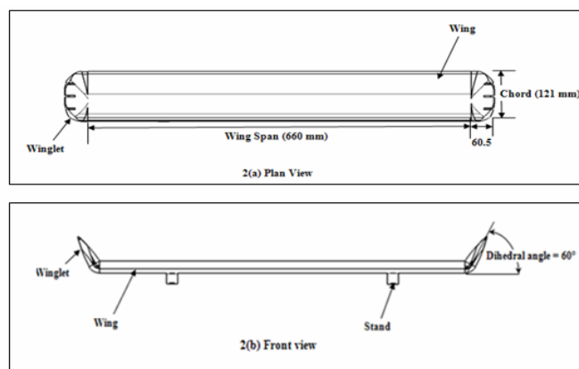
Fig. 2. Rectangular Wing with Winglet using Adapter
