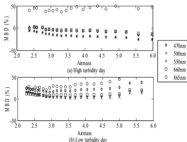
Fig. 4 Performance of Langley calibrated results for (a) high turbidity day (b) low turbidity day
