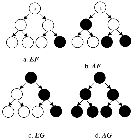
Fig. 13 Basic CTL Operators
