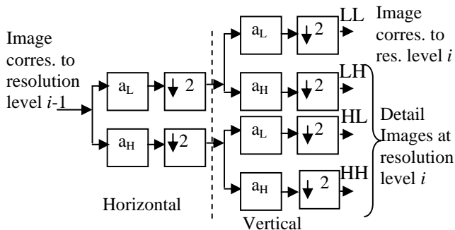
Fig. 1 One Filter Stage in 2D DWT
