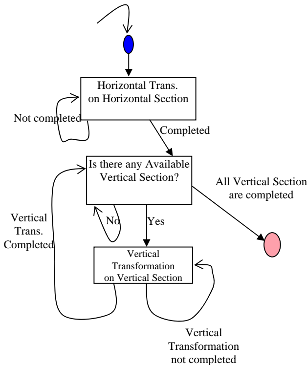
Fig. 14 State diagram of a thread
