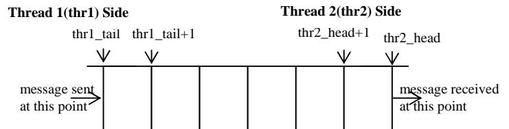
Fig. 15 Channel for message from thread 1 to thread 2
