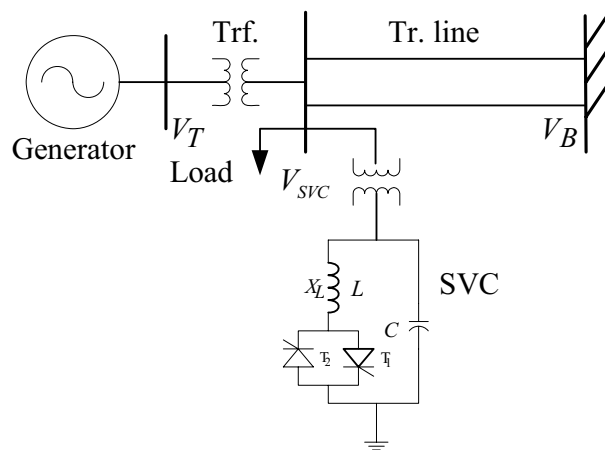
Fig. 5. Single-machine infinite-bus power system with SVC
