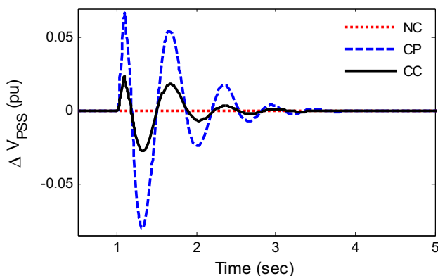
Fig. 11. Stabilising signal of PSS for Case-II
