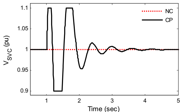
Fig. 9. SVC reference voltage signal for Case-I
