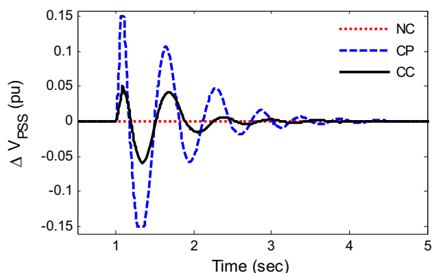
Fig. 14. Stabilising signal of PSS for Case-III
