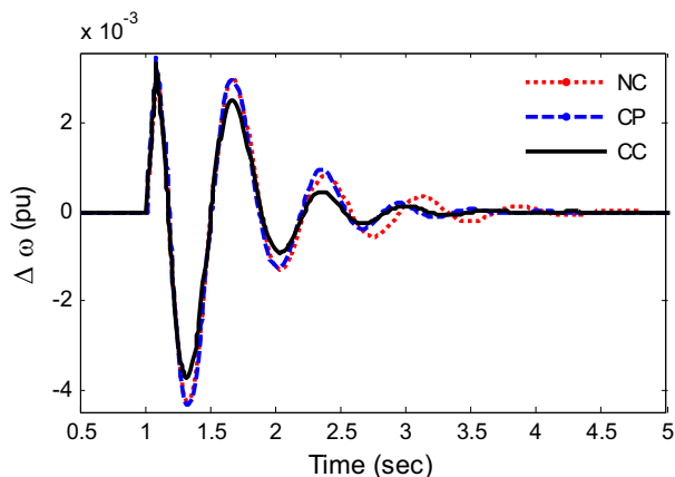
Fig. 10. Speed deviation response for Case-II
