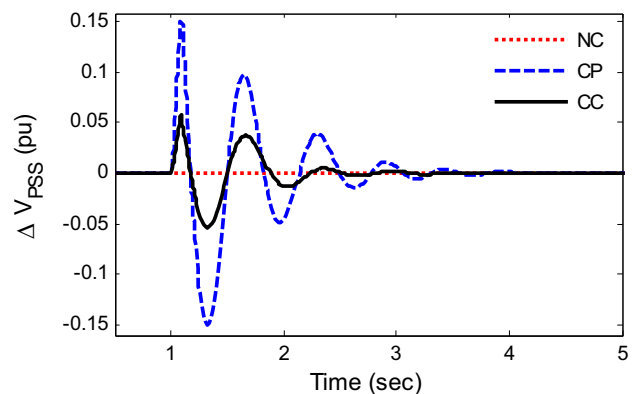
Fig. 8. Stabilising signal of PSS for Case-I
