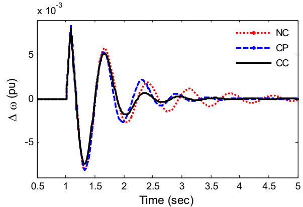
Fig. 6. Speed deviation response for Case-I
