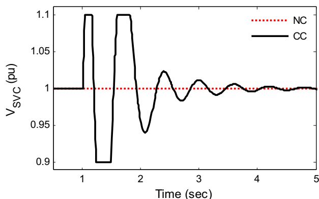
Fig. 15. SVC reference voltage signal for Case-III
