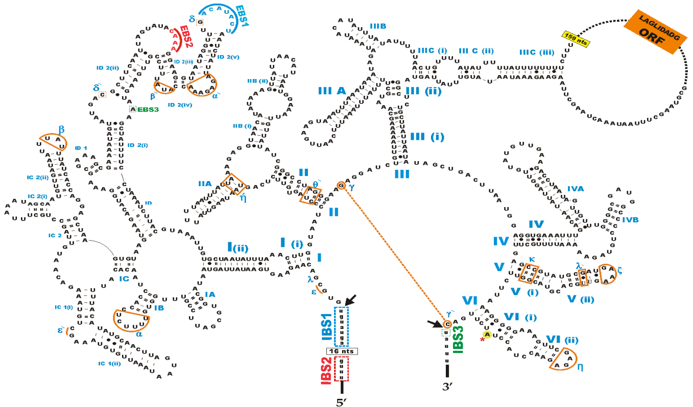
Fig. 2 The secondary structure of the O.ul.mS952 group II B1 intron RNA. Intron sequences are in upper-case letters and exon sequences are in lower-case letters. The positions of EBS1, EBS2 and EBS3 are noted. The positions of IBS1, IBS2 and IBS3 in the 5' and 3' exons are boxed with dotted lines. Tertiary interactions are indicated by dashed lines and Greek letters ( \epsilon , \lambda , \alpha , \beta , \theta , \kappa , \zeta , and \gamma ). The six major structural domains are indicated by Roman numbers (I, II, III, IV, V and VI). The solid black arrows indicate the intron-exon junctions (5' and 3' splicing sites). The asterisk shows the bulged adenosine nucleotide in domain VI (the branch point). The LAGLIDADG ORF is encoded within DIII
