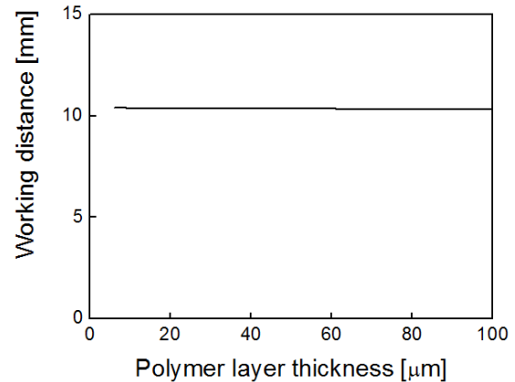
Fig. 4: Working distance vs. polymer layer thickness in the proposed fiber lens structure.
