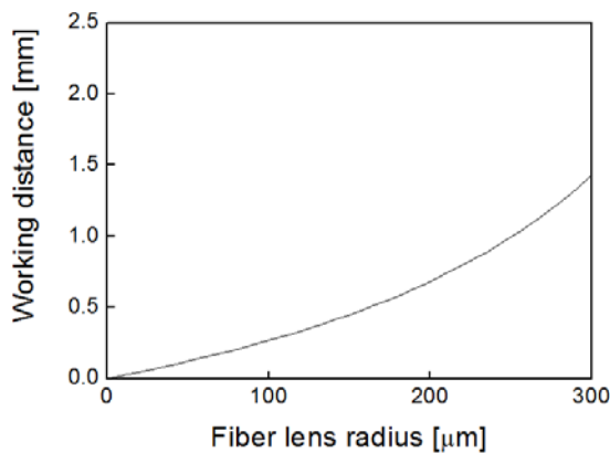
Fig. 2: Working distance vs. radius of fiber lens without polymer layer.
