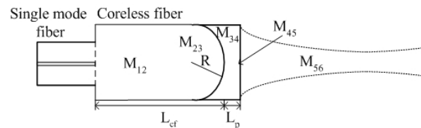
Fig. 1: The proposed fiber lens structure.
