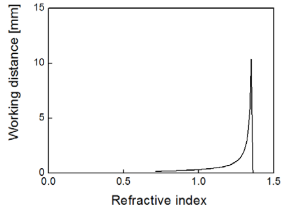
Fig. 3: Working distance vs. refractive index of the polymer layer with thickness of 30 \mu m in the proposed fiber lens structure.
