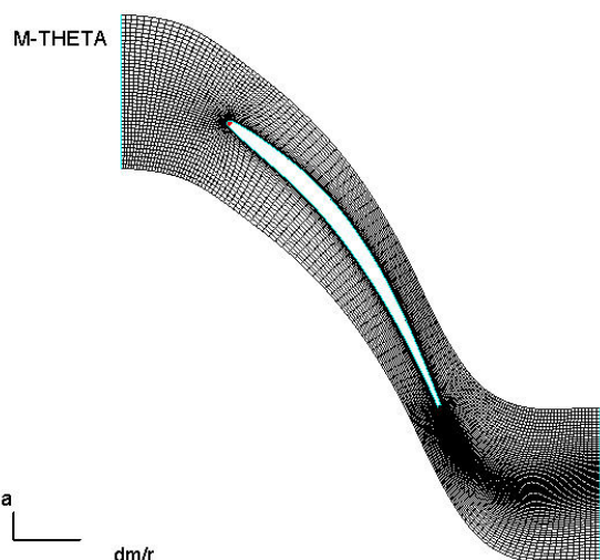
Fig. 5 Blade to blade mesh view at section 4 of an initial runner blade
