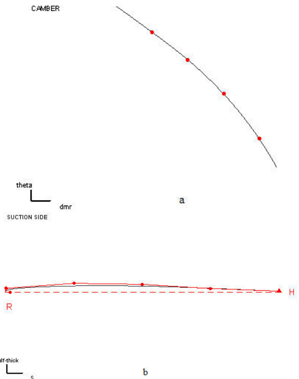
Fig. 4 a) B-spline curve with 5 parameters for each section, b) Bezier curve with 5 parameters for thickness distribution at each section
