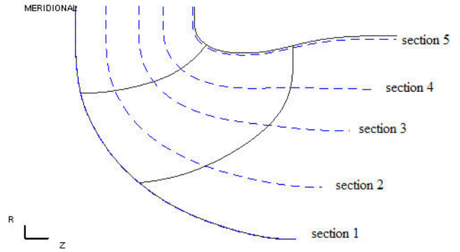
Fig. 3 Geometrical information of GAMM runner turbine
