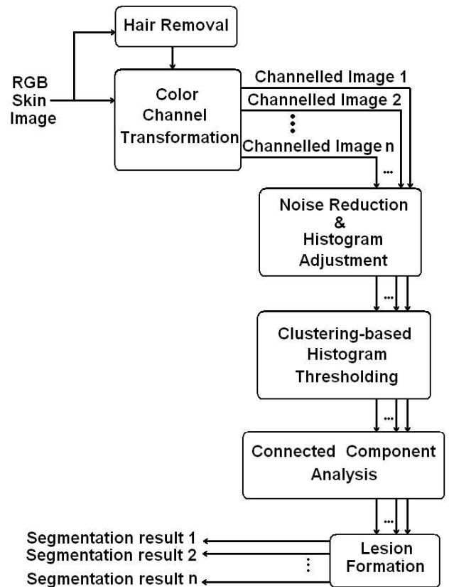
Fig. 1. Segmentation process diagram
