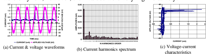
Fig. 2. Typical waveform of low RH clean specimen
