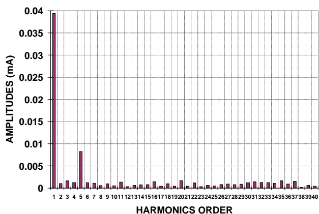
(b) Current harmonics spectrum
