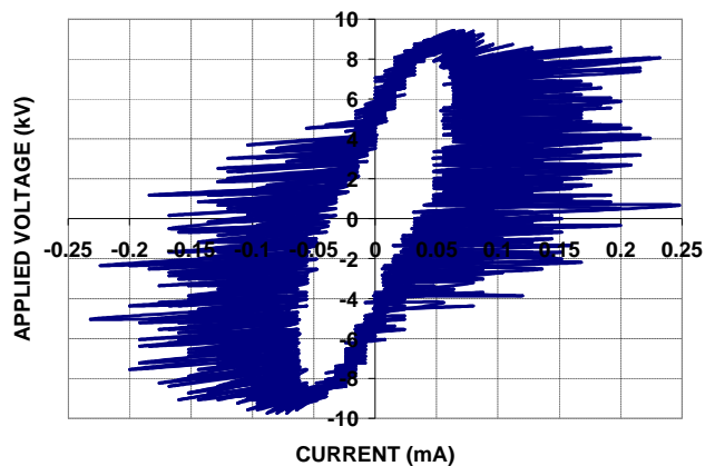
(c) Voltage-current characteristics
