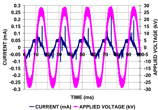
(a) Current & voltage waveforms
