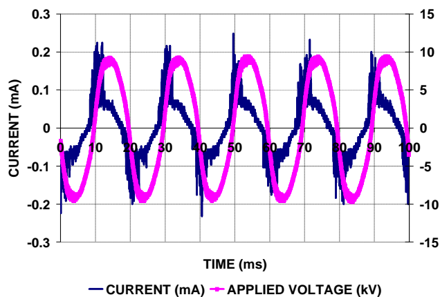
(a) Current & voltage waveforms
