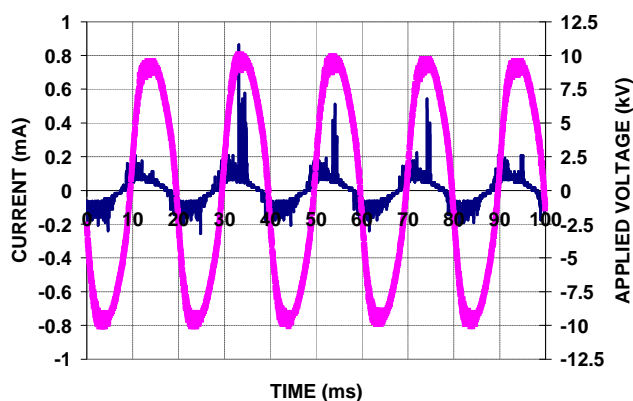
(a) Current & voltage waveforms
