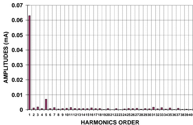
(b) Current harmonics spectrum
