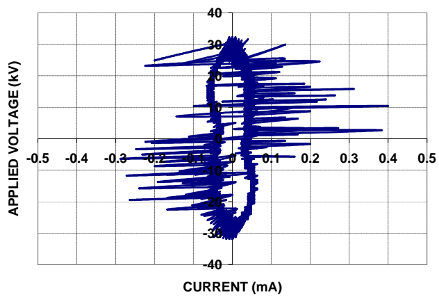
(c) Voltage-current characteristics Fig. 4. Typical waveform of low pressure clean specimen
