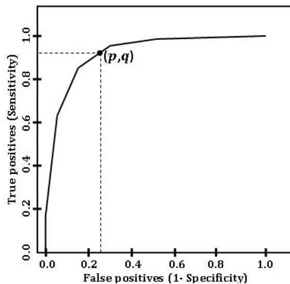
Fig. 1 ROC Curve
