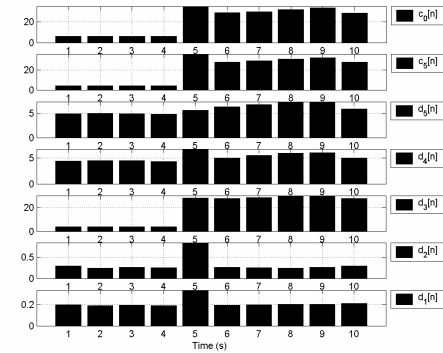
Fig. 6 XLPE conductor phase A HIF on gravel: 95% confidence internal threshold of wavelet coefficients of 3I_0 rms current
