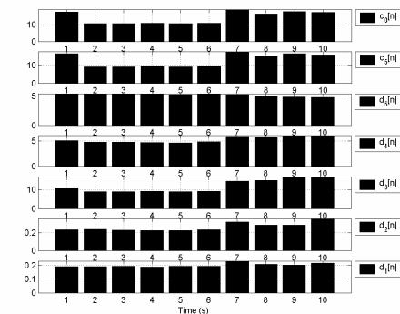
Fig. 3 XLPE conductor phase A HIF on shrub: 95% confidence internal threshold of wavelet coefficients of 3I_0 rms current
