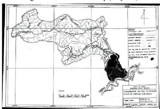
Fig. 4 Flood inundation map (50 years)
