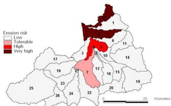
Fig. 2 Spatial distribution of sediment yield predicted by SWAT in the Sarrath catchment
