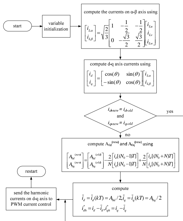
Fig. 2 Flowchart of the DQF method
