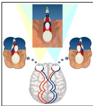
Fig. 2 Binocular Vision
