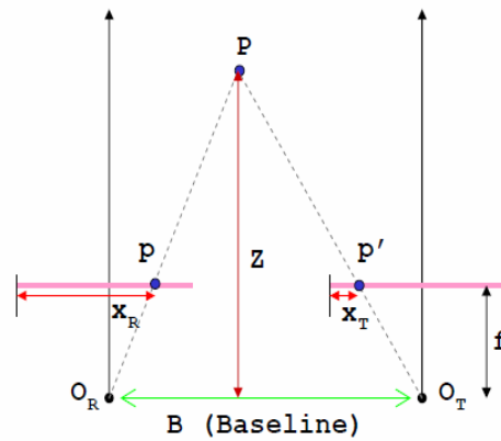
Fig. 4 Epipolar Geometry
