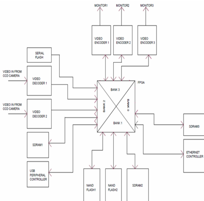
Fig. 5 Block Diagram of Hardware
