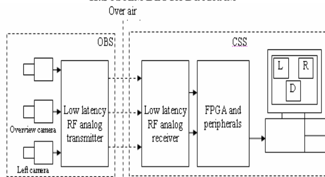
Fig. 1 Block Diagram of Overall System
